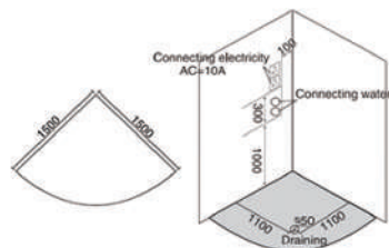
LW-S3813 Size: 1400x1400x2150mm 1500x1500x2150mm 1600x1600x2150mm
