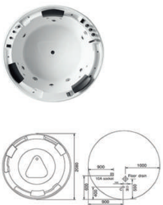
LW-0206 Size: 1600x1600x740mm 1800x1800x740mm 2080x2080x840mm
